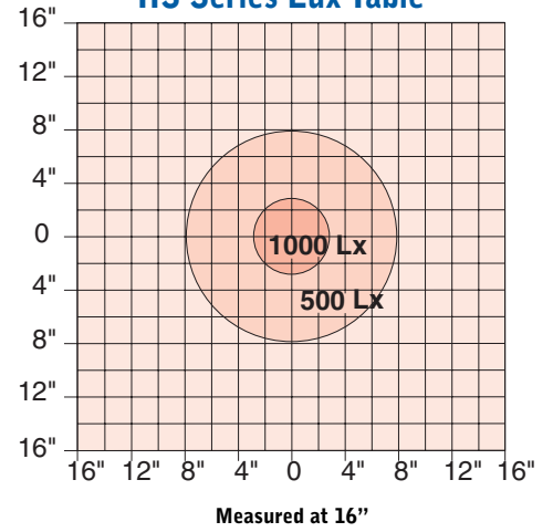
HS Series Lux Table
