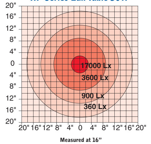
HF Series Lux Table 50W
