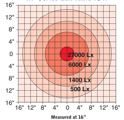
HF Series Lux Table 75W
