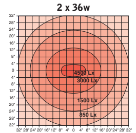
All Measured at 16"
